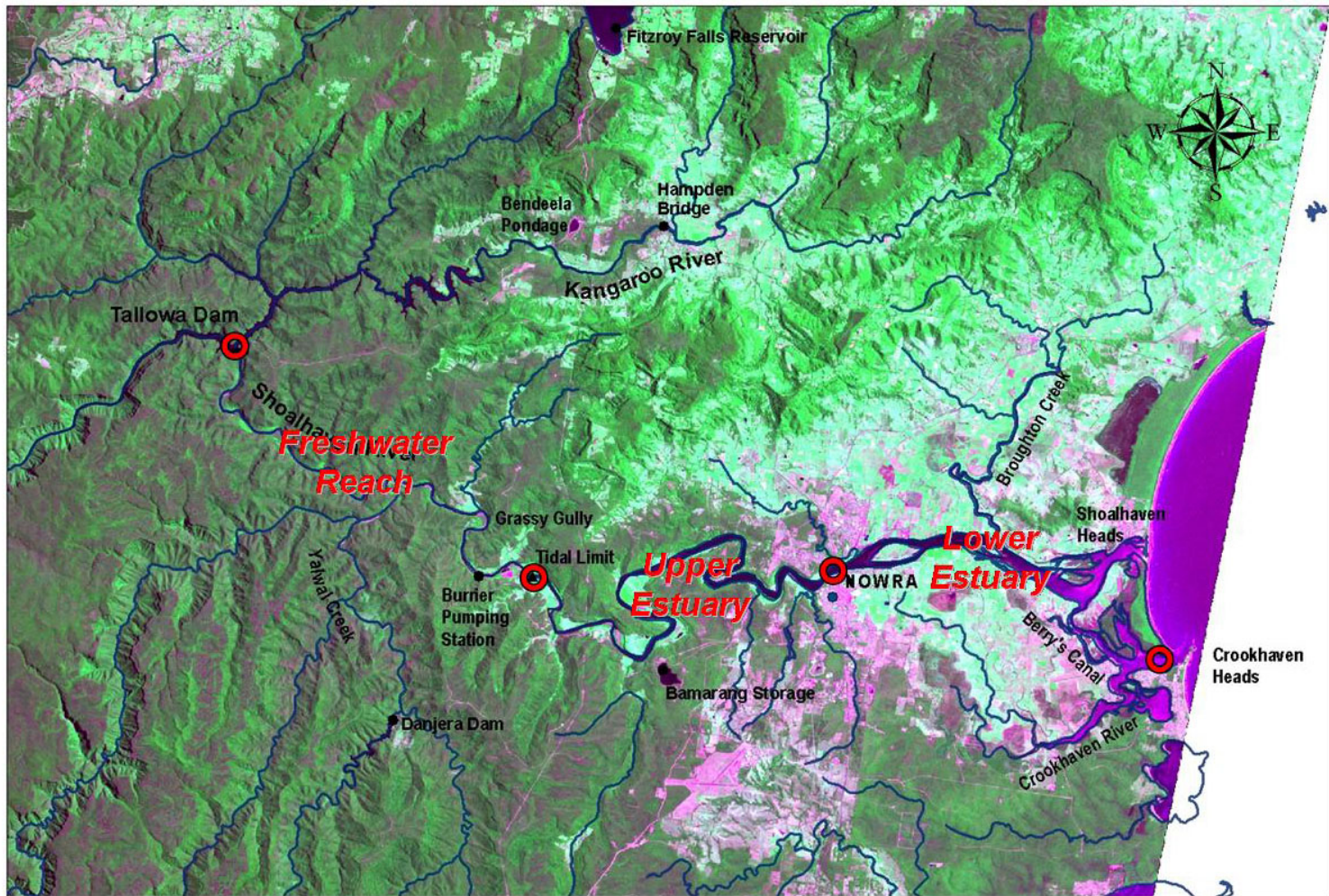
Landsat image of Shoalhaven River d/s Tallowa Dam
